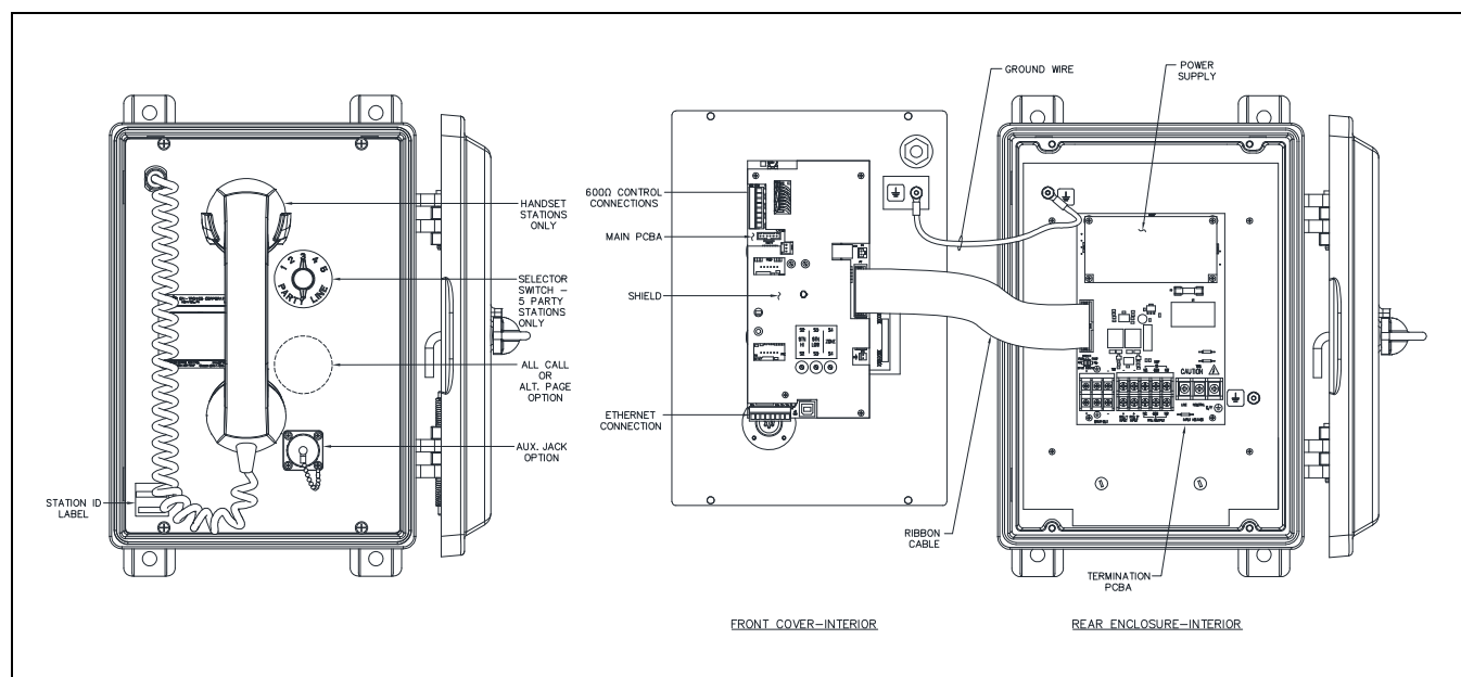
Figure 1. SP2 Weatherproof Handset/Speaker Amplifier Station
